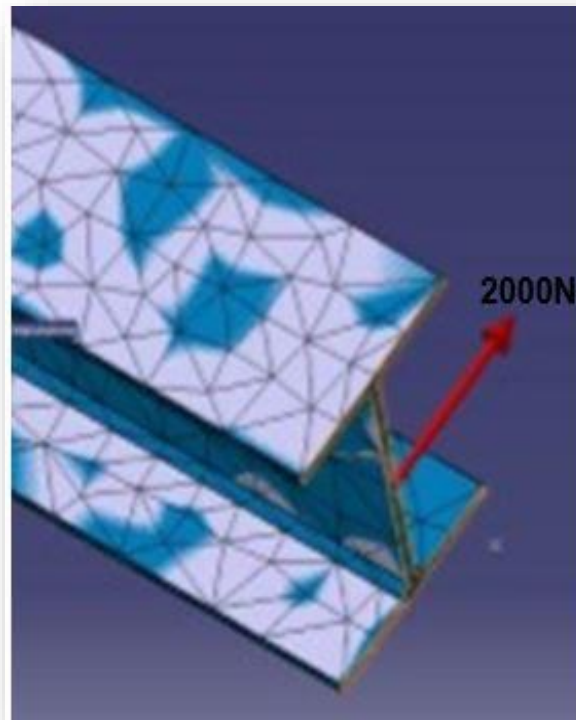
Figure 9 Bending's Force
