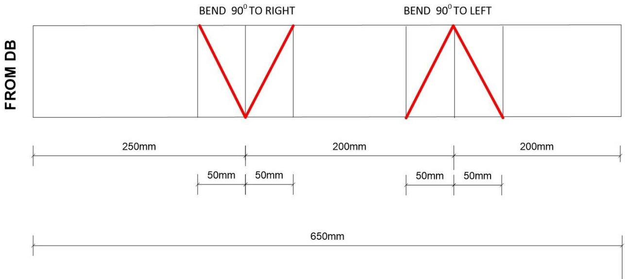
Fig. 7 PVC trunking diagram
